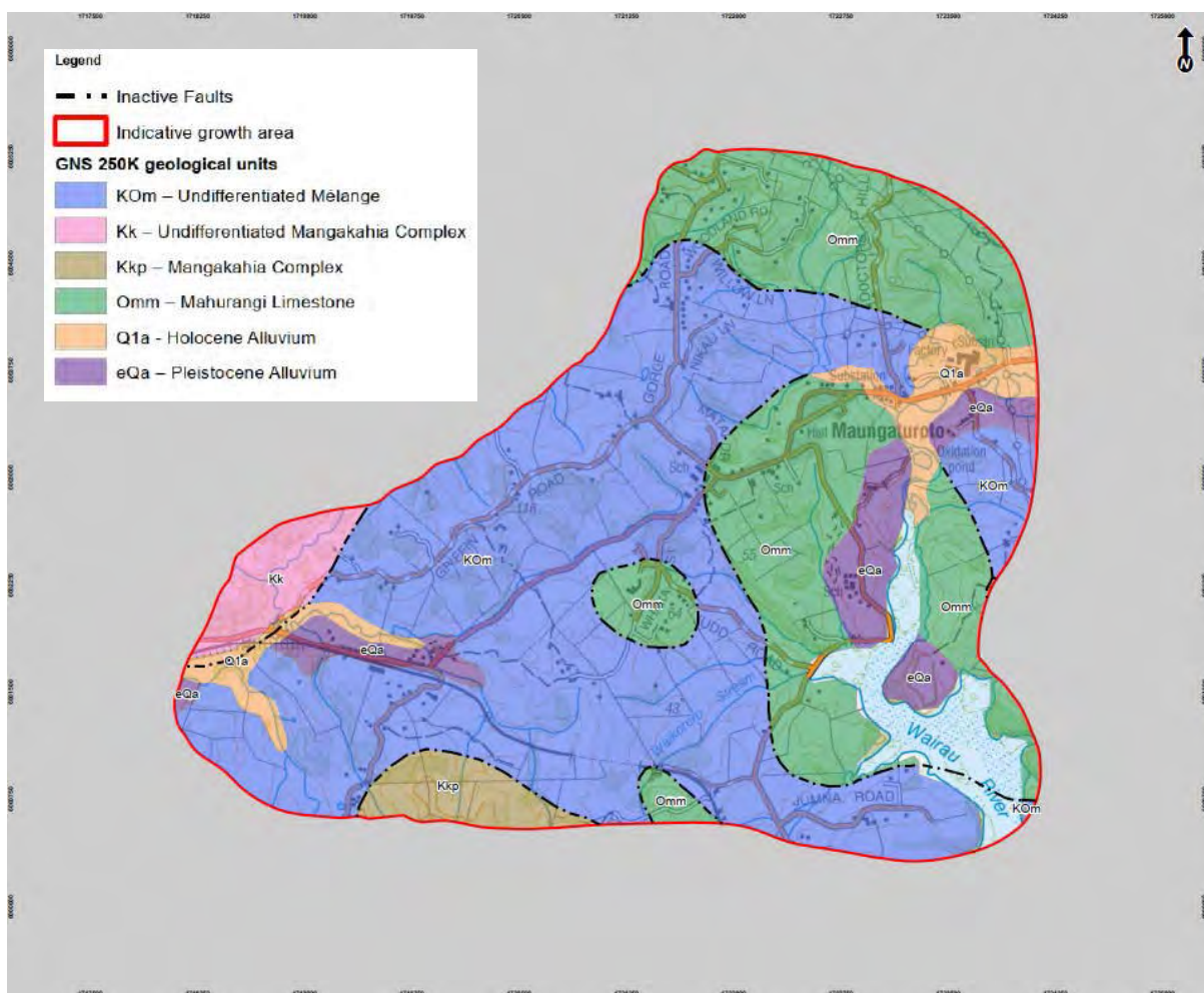
Figure 3: Geology Map
